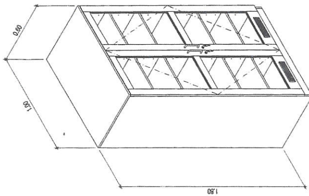
ESC-100 Equipment Storage Cabinet
