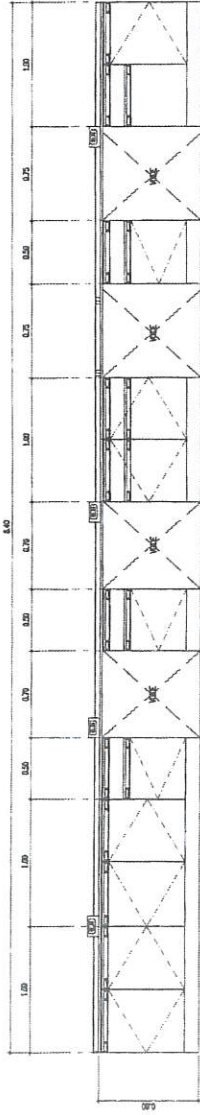
FRONT ELEVATION
